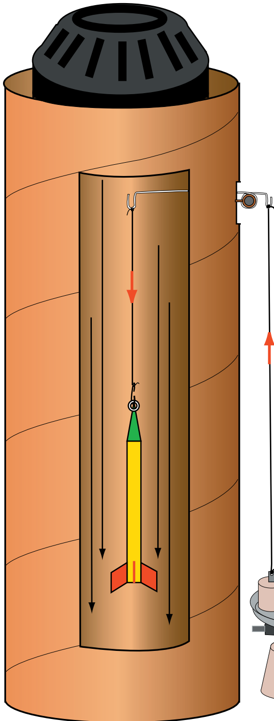
Cutaway view of the tunnel interior (The actual door should be smaller.)
